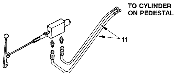
AIR PIPING CIRCUIT
