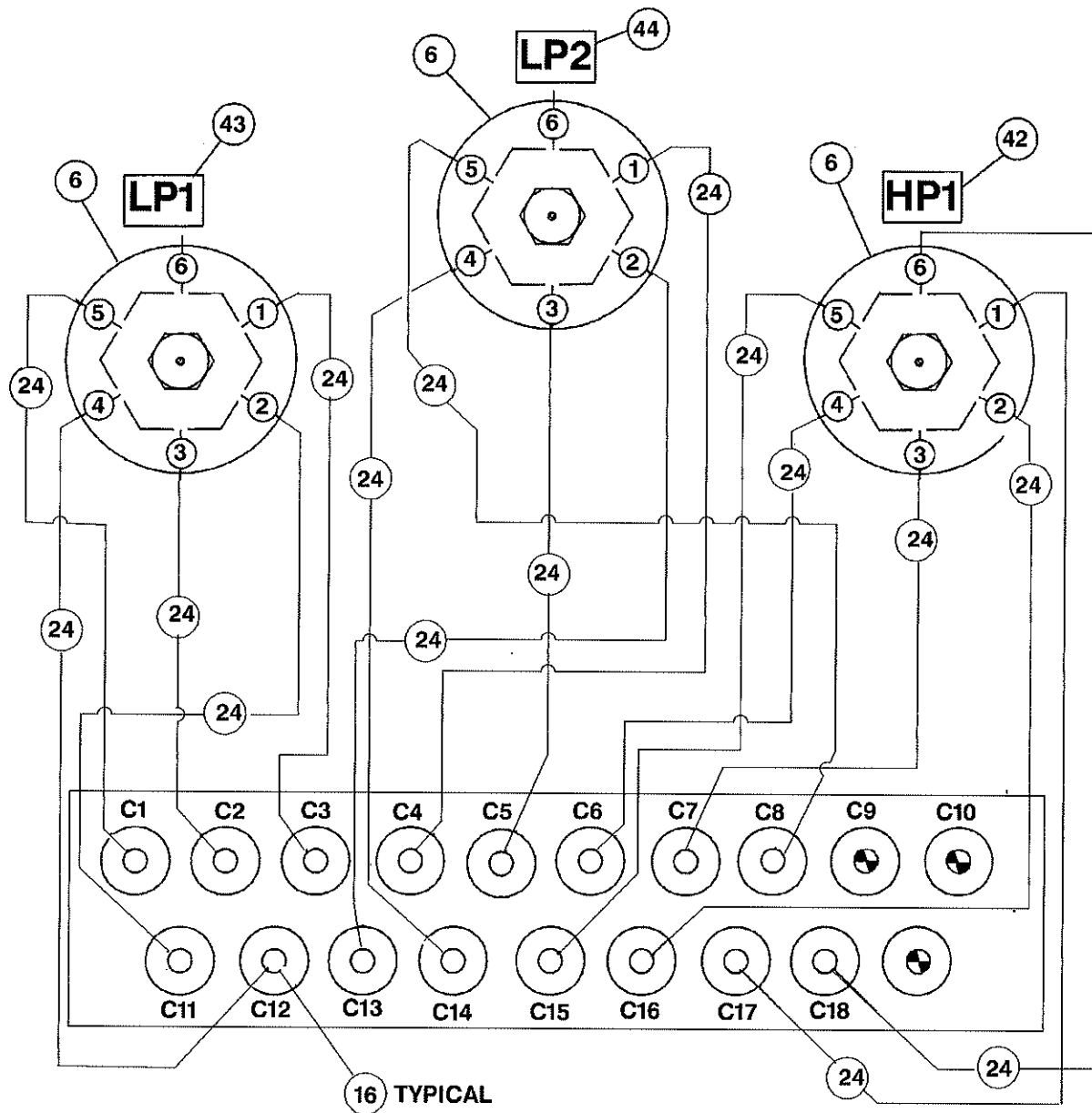
TOP VIEW OF PORT MANIFOLD INDICATING TUBE DESTINATION
